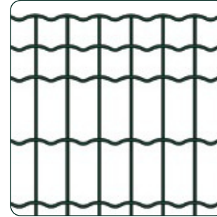
Maille 100x50
